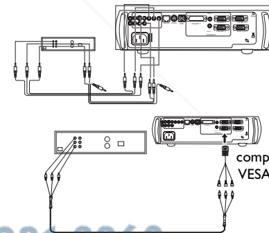
connect component cables and video cables
