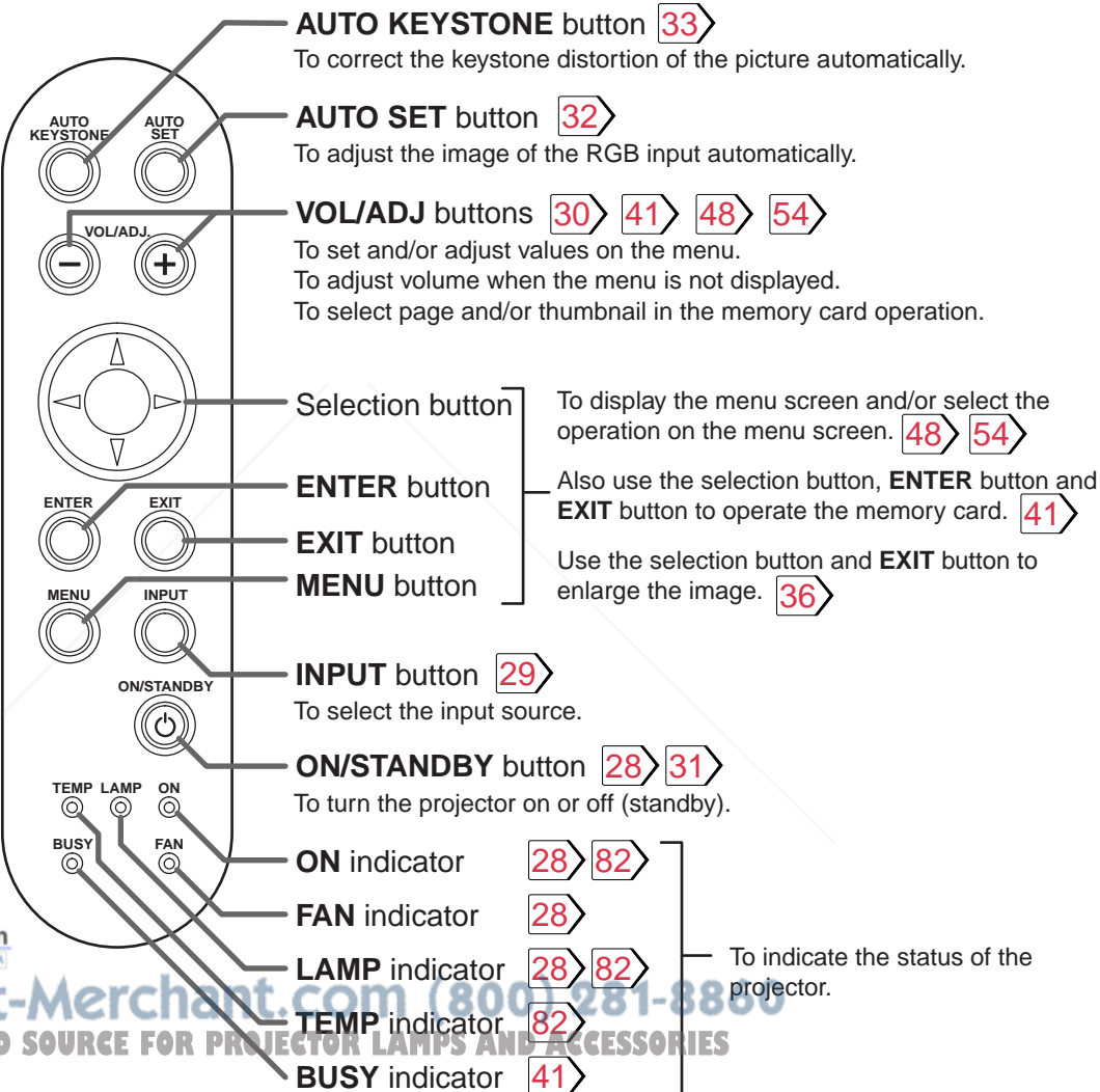
Control panel
