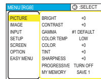
Advanced MENU
