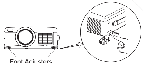
Foot Adjusters
