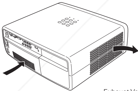
Air Intake Vent
