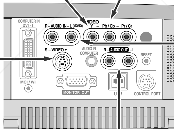
Terminals of the Projector
