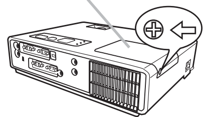
The lamp cover
