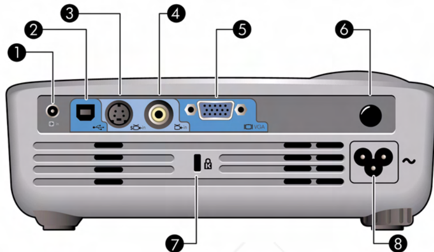
Identifying back panel components
