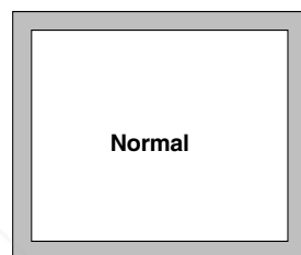
Keystone distortion
