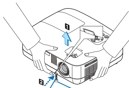
Adjustable Tilt Foot Lever Adjustable Tilt Foot
