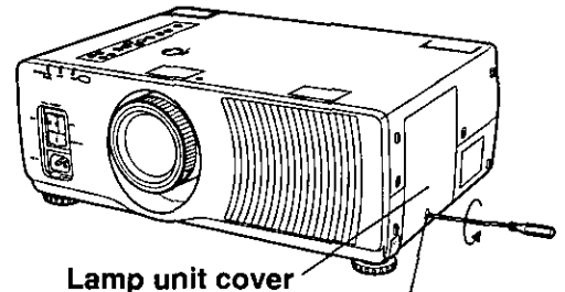
Fixing screw for the lamp unit cover
