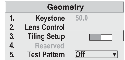
Figure 3.21. Geometry Menu
