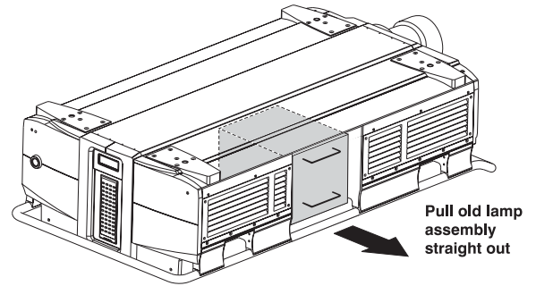
Figure 4.5. Pull out old lamp module
