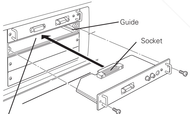
Figure shows D-sub 15 terminal.
